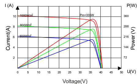
Current-Voltage&Power-Voltage Curve(335W)
